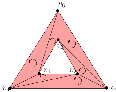
Figure 7.4: One- and two-chains in an annulus.
