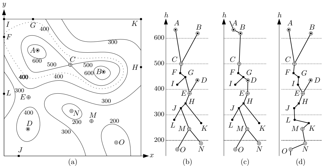
Figure 7.15: (a) a contour map of level sets (isolines), (b) the corresponding contour tree, (c) the join tree, and (d) the split tree. As in Fig. 7.14, minima and maxima are indicated by empty and full circles, and crosses denote saddle points. The points where a contour touches the boundary play also a role in the contour tree (for example, they may be local minima or maxima) but they are not critical points in the sense of having derivative 0. The level sets in (a) are labeled with the height values, and these values are indicated in the trees of (b), (c), and (d). The critical point F changes only the topology of a contour and not the number of contours; when the contour tree is viewed as a discrete structure, F is not a vertex of the tree.
