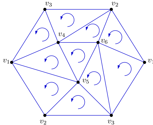
Figure 7.10: A triangulation of the projective plane.
