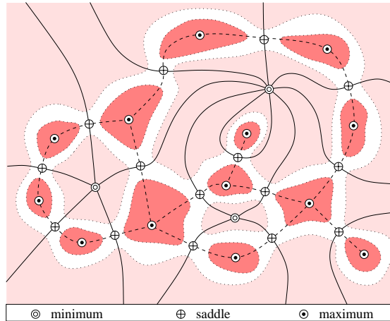
Figure 7.14: The Morse-Smale complex of a function on the plane. The stable one-manifolds are solid, the unstable one-manifolds are dashed. (Courtesy Herbert Edelsbrunner.)
