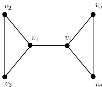
Figure 7.5: Zero-homology of a graph.
