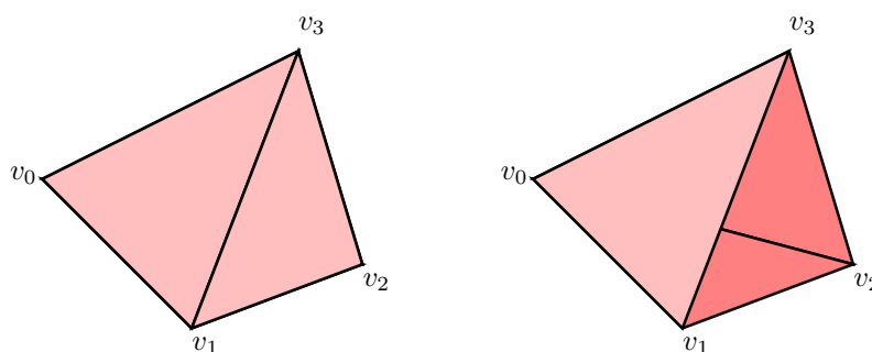
Figure 7.9: An elementary collapse removes the simplices v_0v_1v_2v_3 and v_1v_2v_3 from the leftmost simplex.
