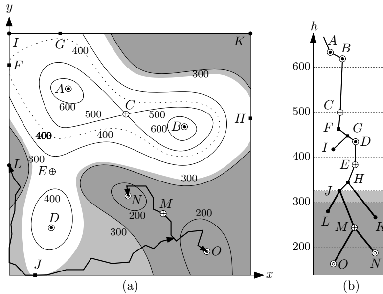
Figure 7.17: Identifying the components that are to be merged by growing descending paths.
