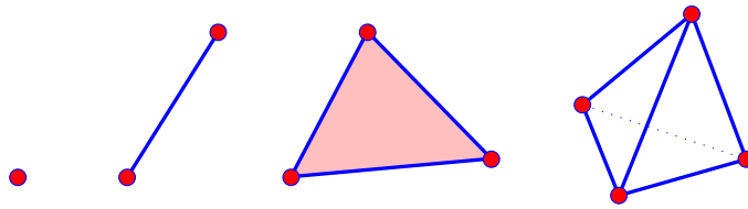
Figure 7.1: Simplicies of dimension zero, one, two and three.
