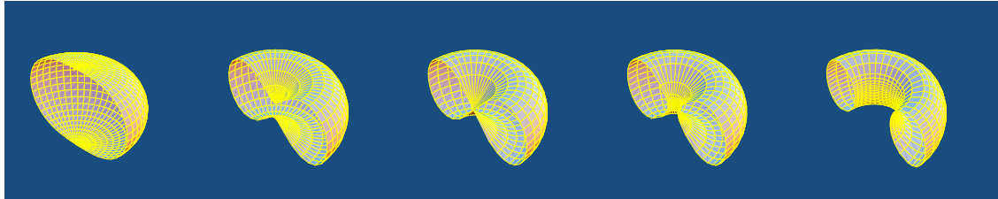
Figure 7.11: Passing a critical level set of a Morse function in three-space. The critical point has index 1. A local model of the function near the critical point is f(x_1, x_2, x_3) = -x_1^2 + x_2^2 + x_3^2 , with the x_1 -axis running vertically.
