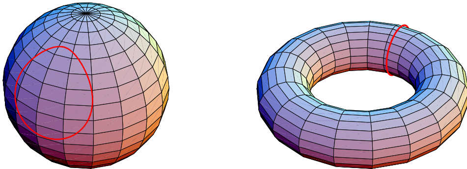
Figure 7.3: Every simple closed curve on the sphere disconnects. Not every closed curve on the torus disconnects.
