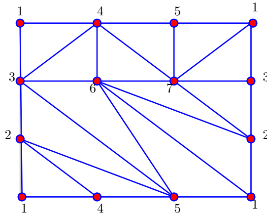
Figure 7.8: A triangulation of the torus.
