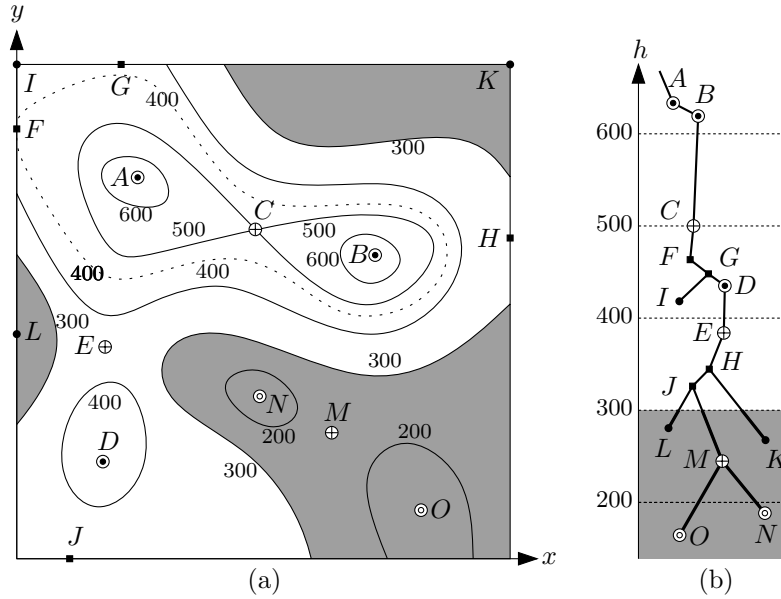
Figure 7.16: (a) the lower level set at level 300 and (b) the corresponding part in the join tree.
