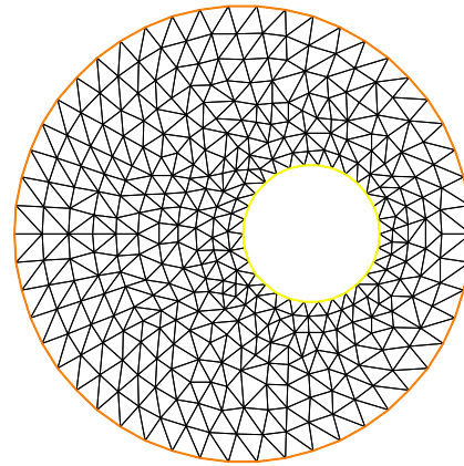
Figure 5.4: mesh with hole
