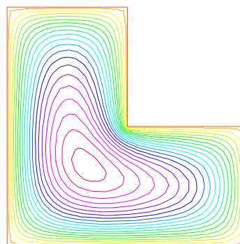
Figure 5.14: Final solution after 4-times adaptation
