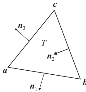
Figure 6.8: normal vectors of each edge
