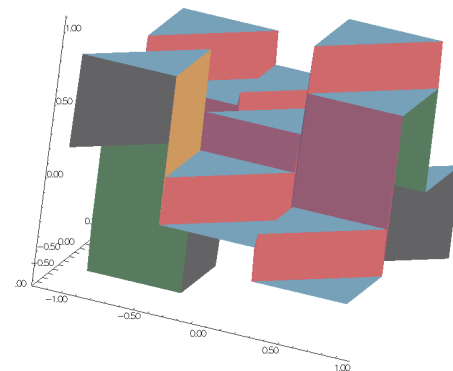
Figure 6.3: projection to V_h(\mathcal{T}_h, \mathbf{P0})
