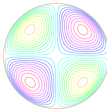
Figure 2.2: isovalues by plot(u)
